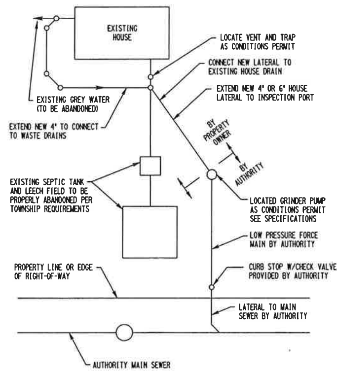
SEPTIC TANK BYPASS PLAN N.T.S.
