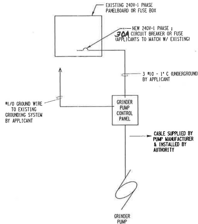
ELECTRICAL ONE - LINE DIAGRAM N.T.S.
