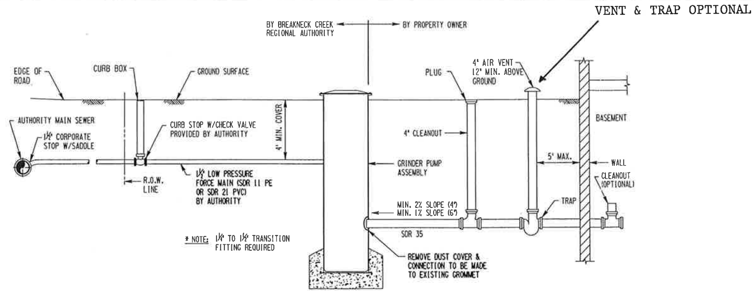
ELEVATION SERVICE CONNECTION N.T.S.
