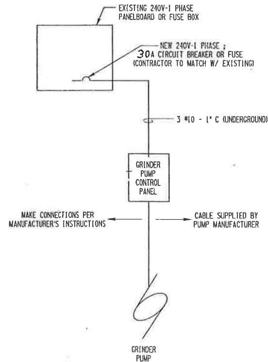
ELECTRICAL ONE - LINE DIAGRAM N.T.S.
