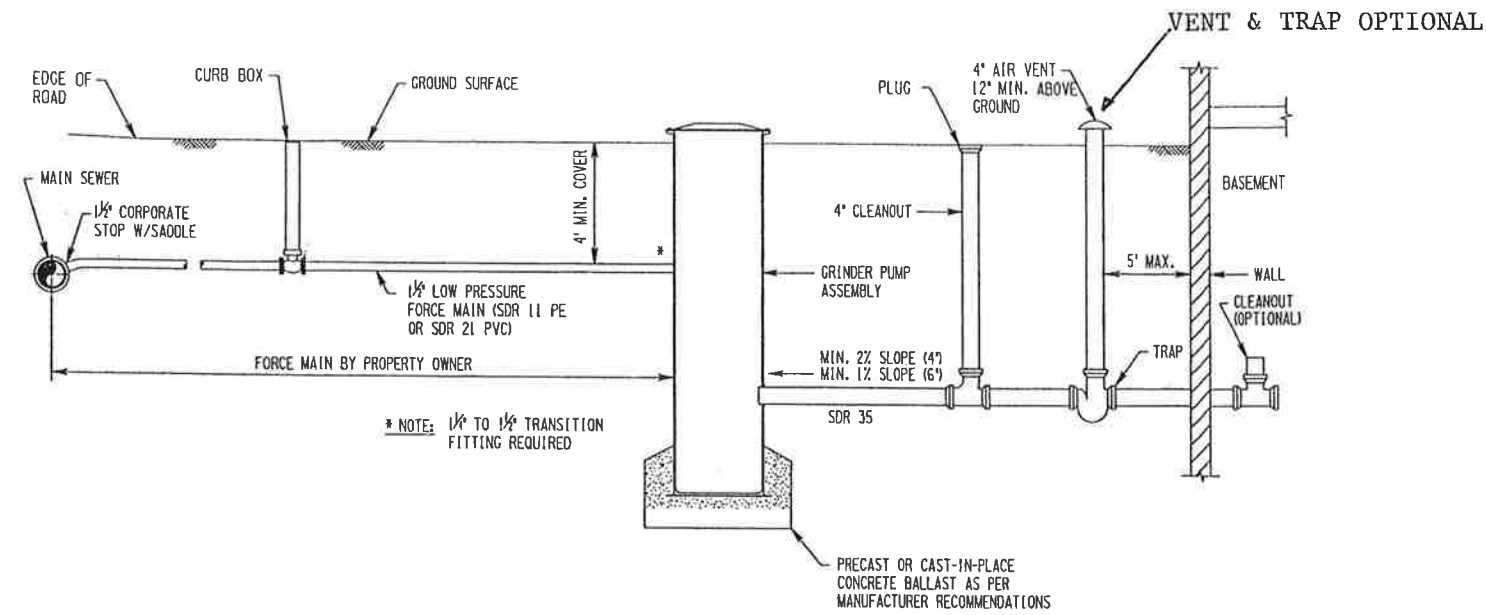
ELEVATION SERVICE CONNECTION
